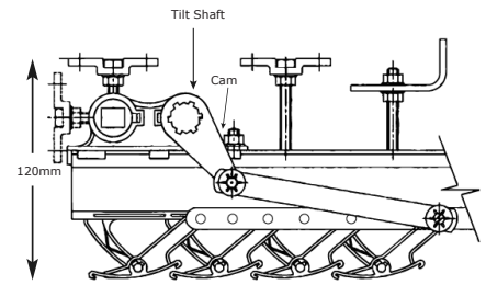
T50 Rack Arm Diagram ii
